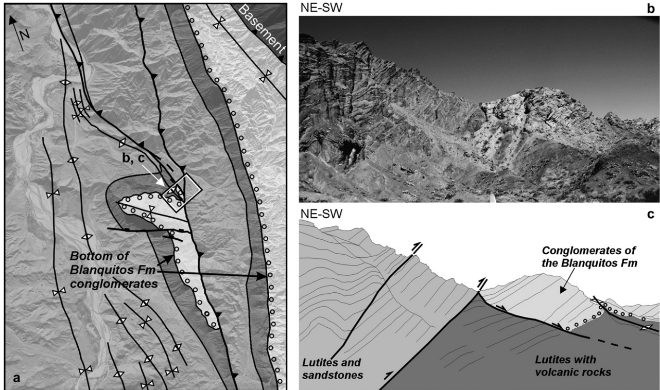
Fig. 5. (a) Structural sketch map north of Rio de las Conchas showing the location and change of orientation of folds and thrusts; these appear controlled by earlier, pre-orogenic extensional faults. (b) Panoramic view of a preserved extensional fault which is truncated by a thrust. This thrust controls the location and the orientation of the anticline in its hanging-wall. See Fig. 4 for location.
